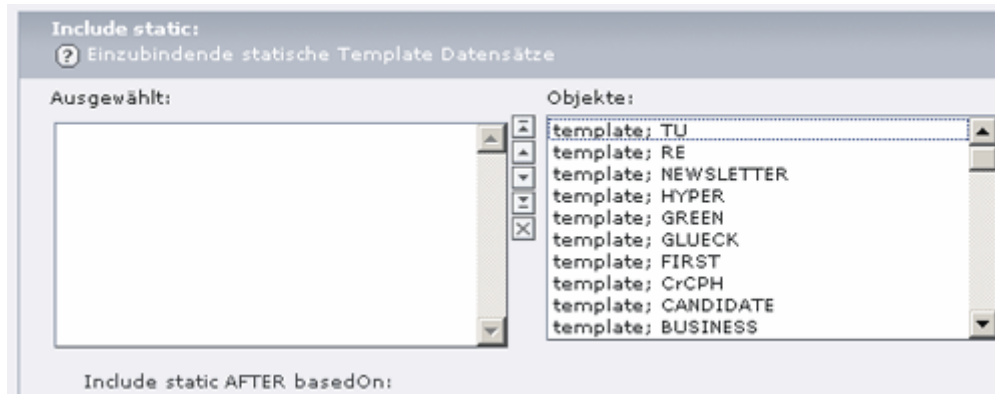
Bild 4: Include Static
